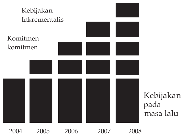
Gambar 8. Model Inkrementalis
